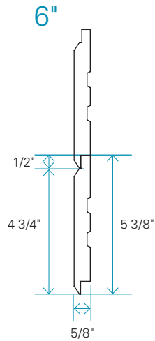
INSTALLATION NAILED ON FURRING STRIPS
